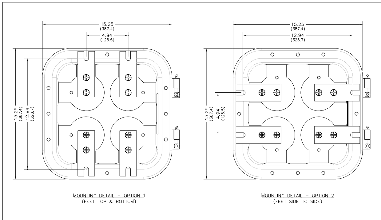
Figure 4. Model 7085-005-UL/EX Enclosure Mounting Details
