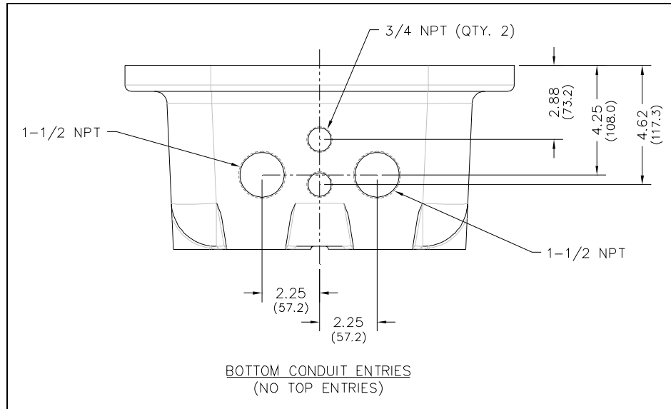
Figure 5. Model 7085-005-UL Conduit Entries
