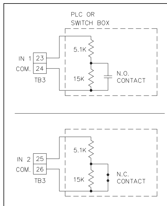
Figure 9. PLC or Switch Box Normally Open and Normally Closed - Example
