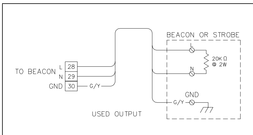
Figure 8. Beacon or Strobe
