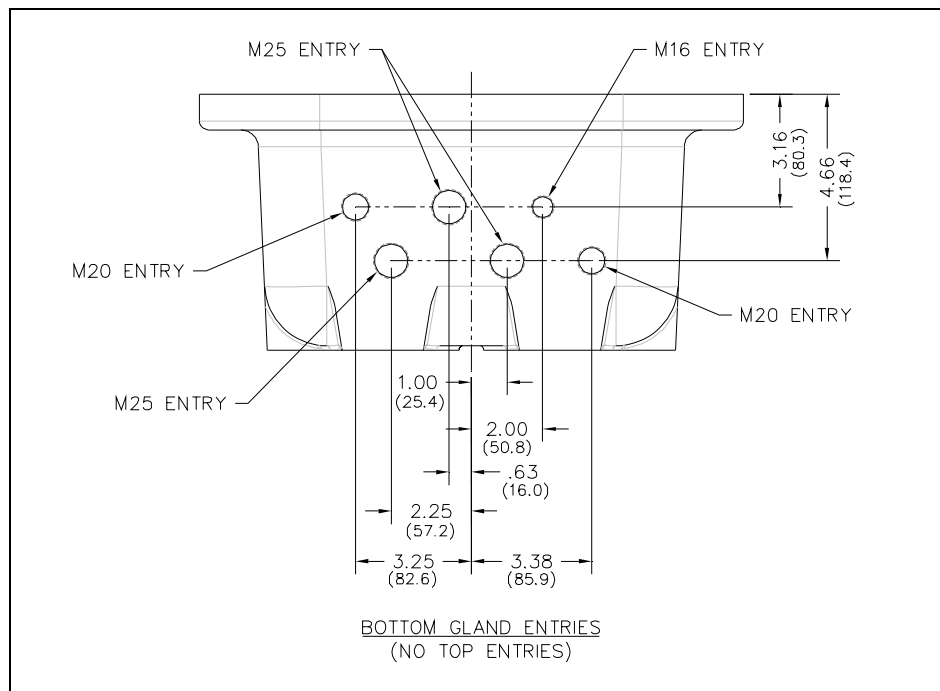
Figure 6. Model 7085-005-EX Cable Gland Entries
