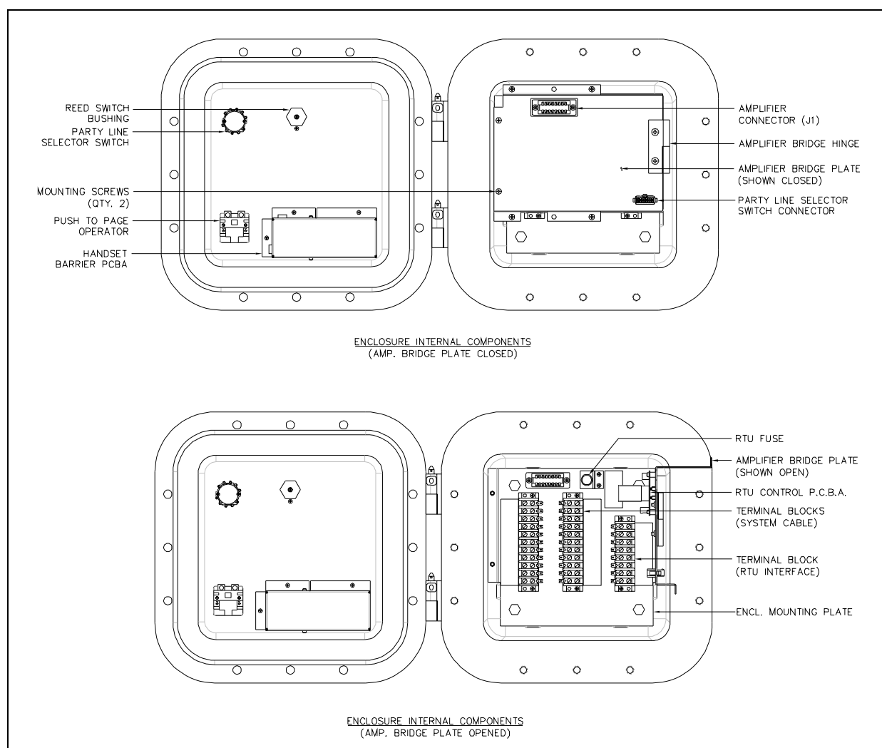
Figure 3. Model 7085-005-UL/EX Amplifier Enclosures interior view
