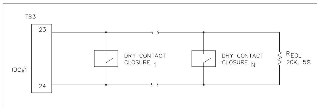
Figure 10. Input Line Supervision Multiple Switch - Example
