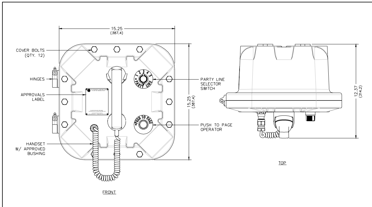
Figure 2. Model 7085-005-UL/EX Outline Drawing
